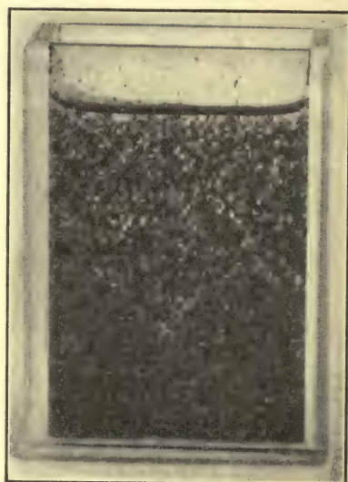
FIG. 6.—Coagulated through addition of 2 per cent. sulphuric acid.
